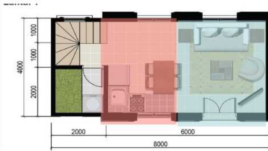
1 st Floor
