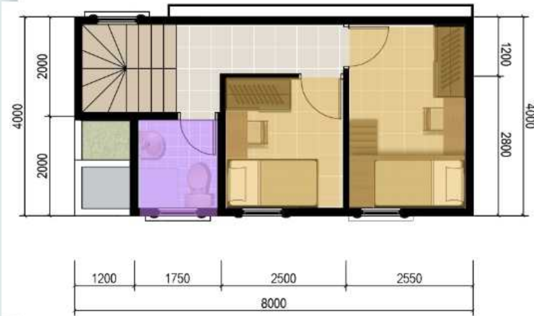
2 nd Floor
