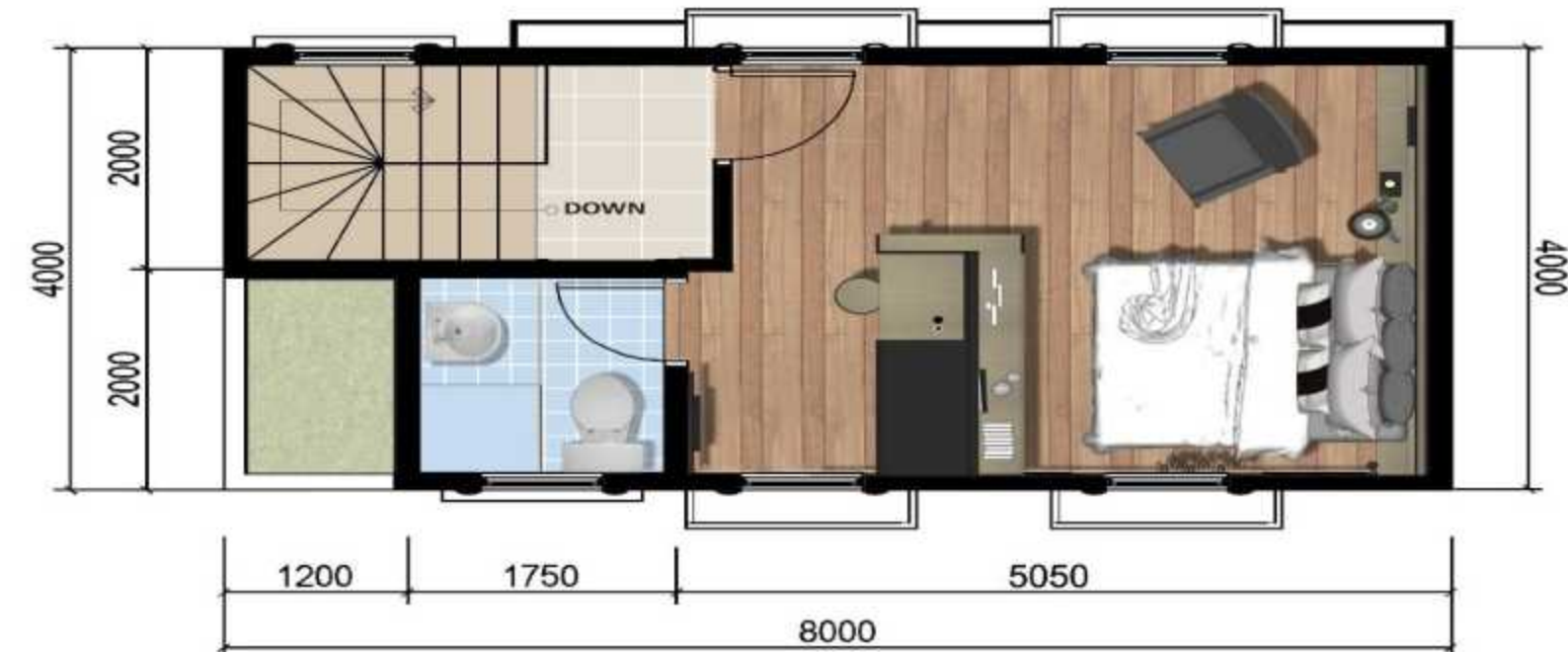
DENAH LANTAI 3
