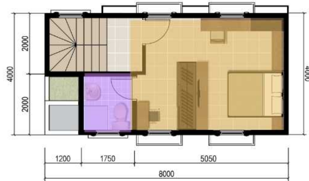
3 rd Floor
