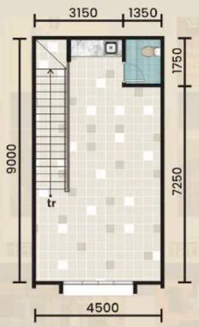
DENAH LANTAI 2
