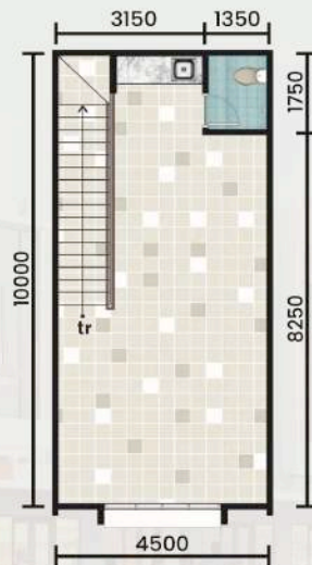
DENAH LANTAI 2
