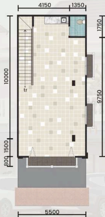
DENAH LANTAI 2
