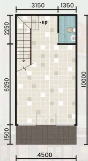
DENAH LANTAI 1
