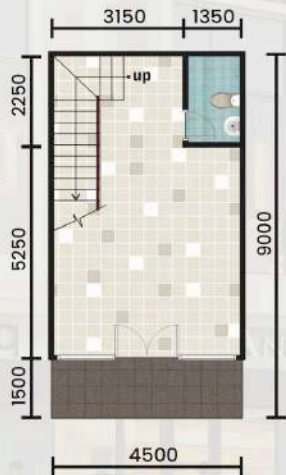
DENAH LANTAI 1
