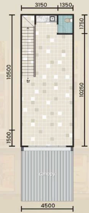
DENAH LANTAI 2
