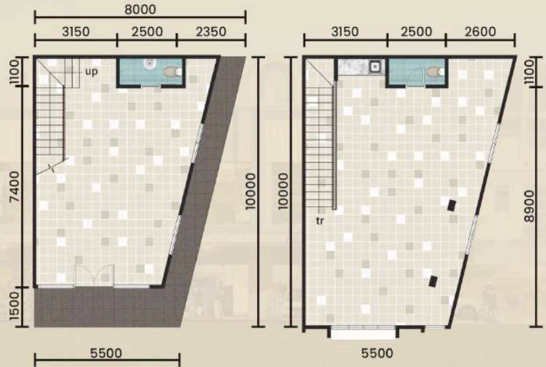
DENAH LANTAI 1
