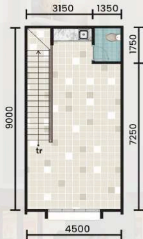
DENAH LANTAI 2
