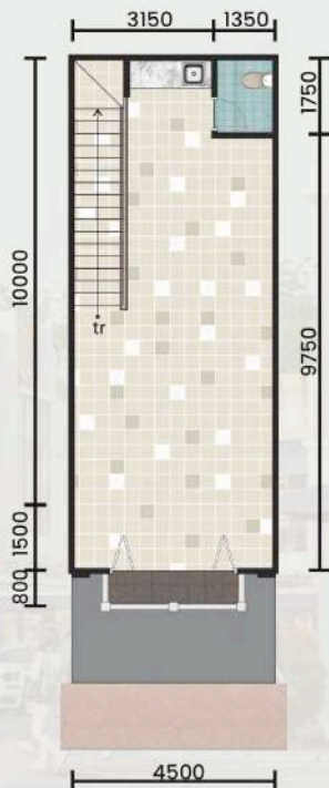
DENAH LANTAI 2
