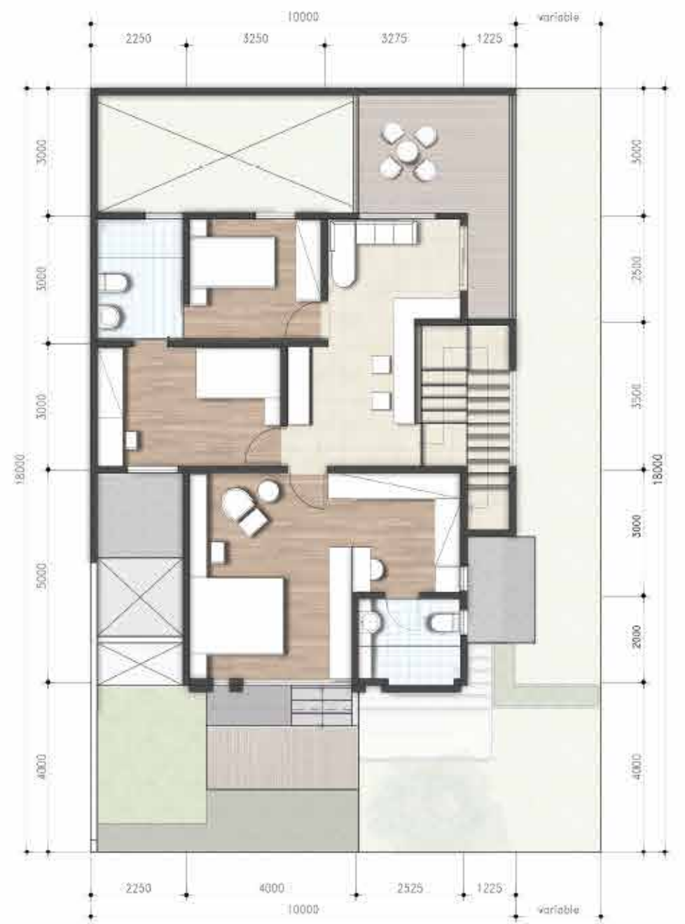
CORNER - SECOND FLOOR
