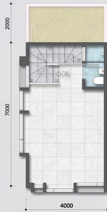
LEVEL 3
