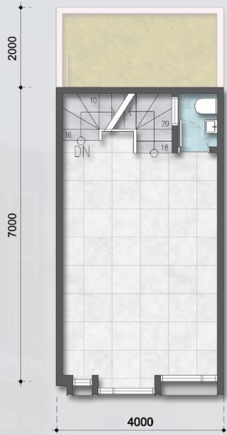
LEVEL 2
