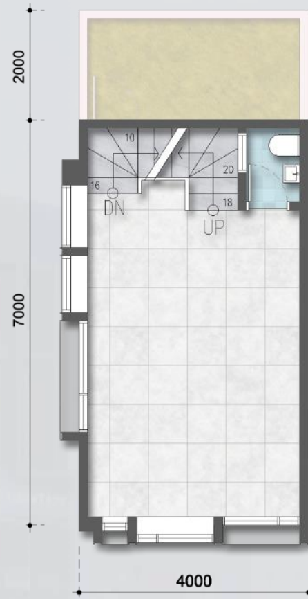
LEVEL 2
